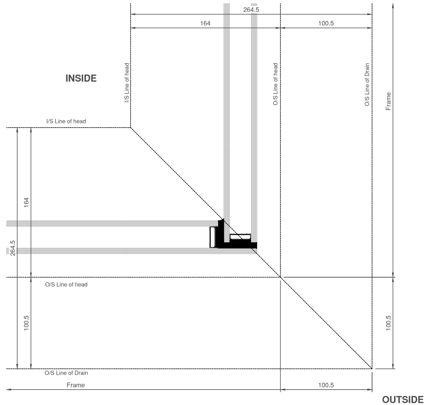
Glass-to-Glass HORIZONTAL SECTION
